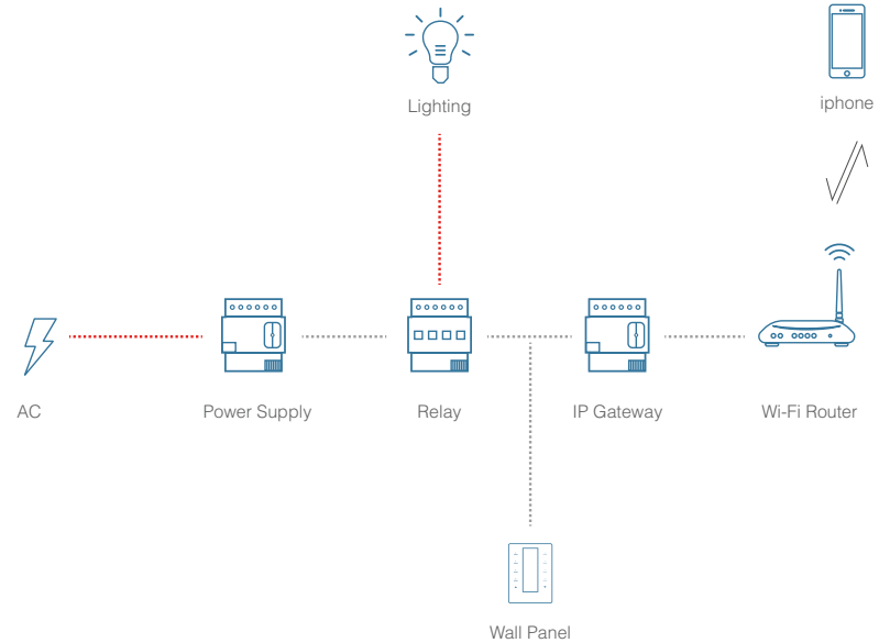
Topology of a minimum Buspro solution
