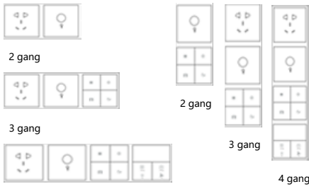
Figure 5. Horizontal installation
