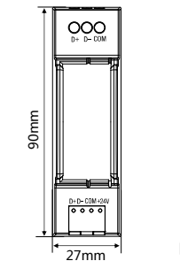
Figure 5. Base - Front View
