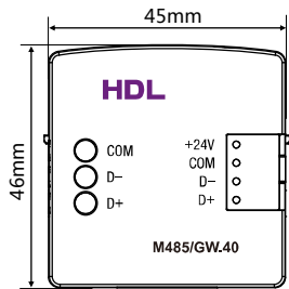
Figure 3. Dimensions - Front View Figure 4. Dimensions - Side View
