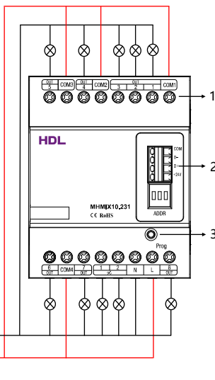
Figure 4. Wiring
